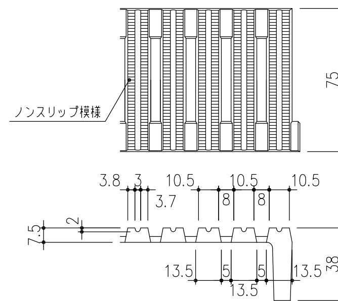
Non-slip detail S=1/2
