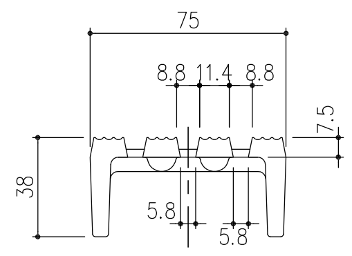
Non-slip detail S=1/2
