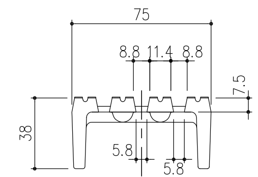
Non-slip detail drawing S=1/2
