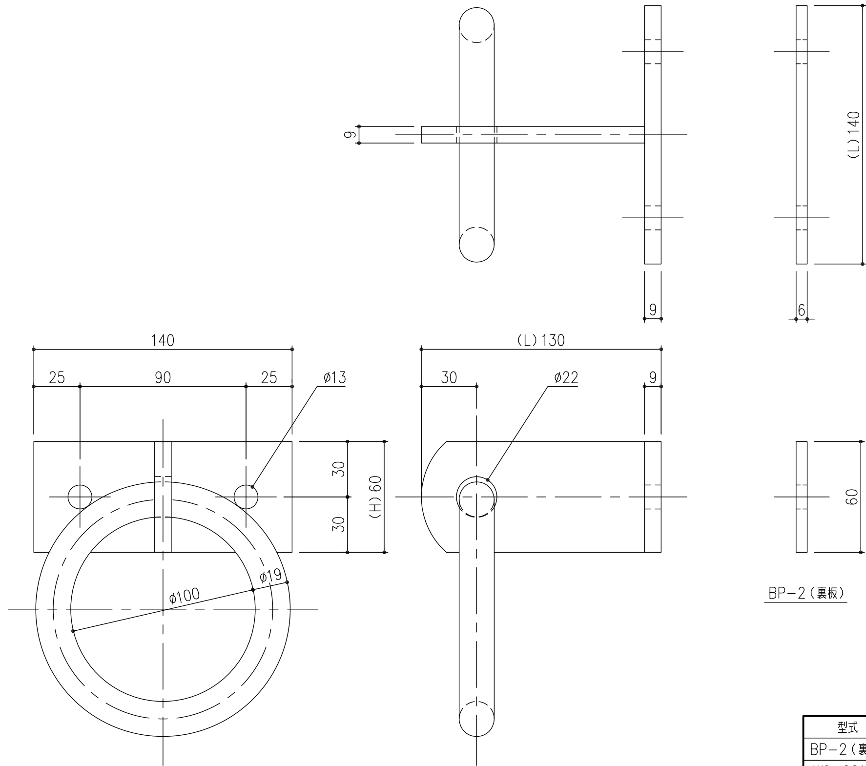
W9-6013S (吊環金具)
