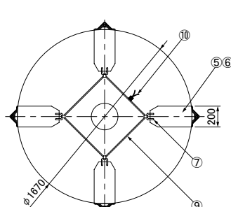
DJP-4S ●質量: 48kg
