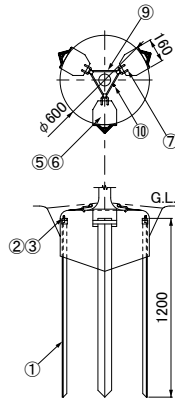
DJP-4S ●質量: 48kg
